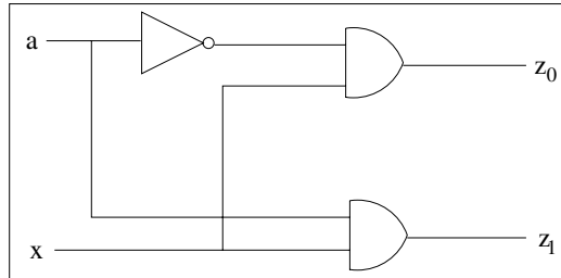
Figure 13.7: Demultiplexor
